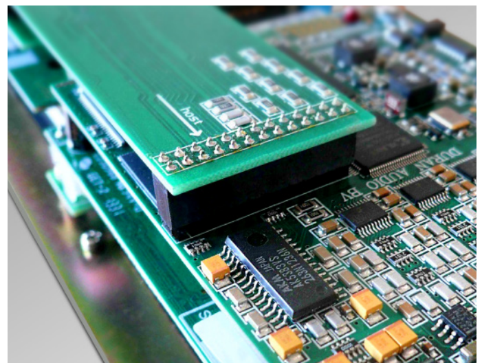
Integrated electronics module which combines powerful Digital Signal Processing with multi-channel class D Amplifiers
